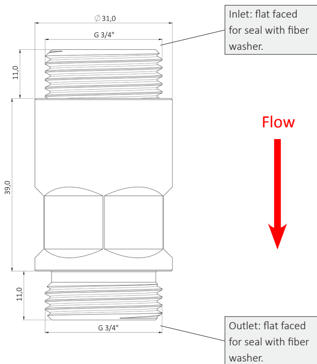
Image: MF Inline 1P 3/4" (dimensions in mm)
